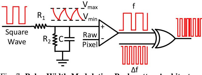
Fig. 7: Pulse Width Modulation Backscatter Architecture.
