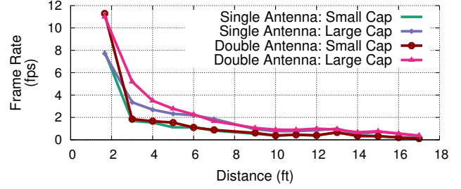
Fig. 8: RF Harvesting Evaluation. Frame rates of our video streaming camera at different distances when it is powered only by the RF harvester. Note that we define the frame rate as average number of frames over a short period of time (a few minutes).
