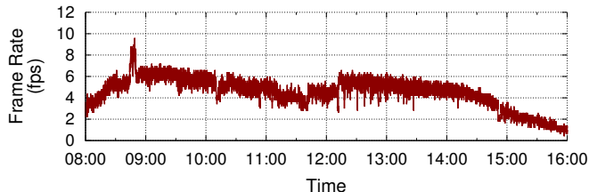
Fig. 14: Application Deployment. Video streaming frame rate achieved by our battery-free video camera over the course of eight hours.
